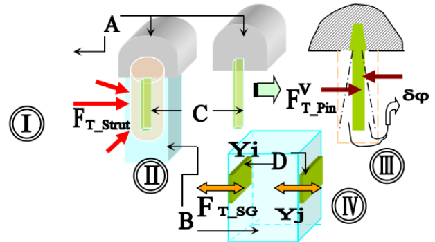
Figure 9. Schematic view of the force transmission route of the robotic sensor system
