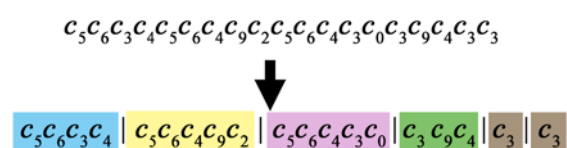
Figure 3 Any string can be split into subsequences
