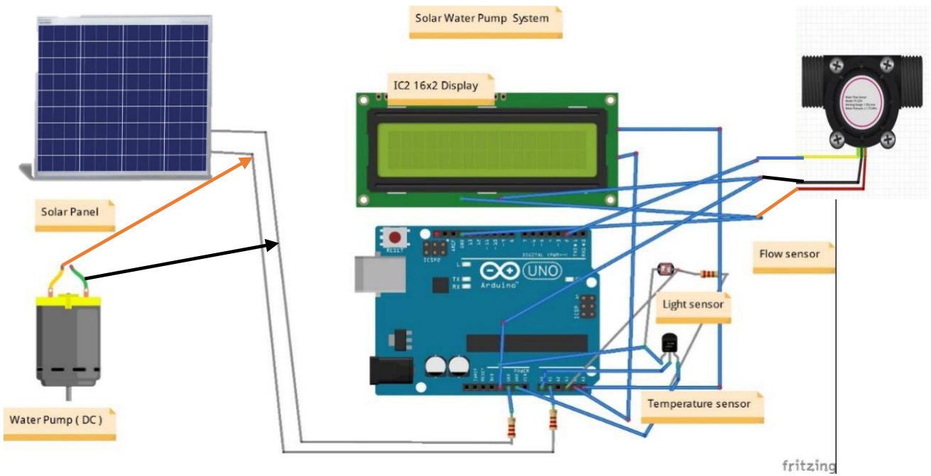
Figure 7. Circuit Diagram
