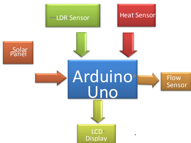
Figure 4. Block diagram of solar powered water pump
