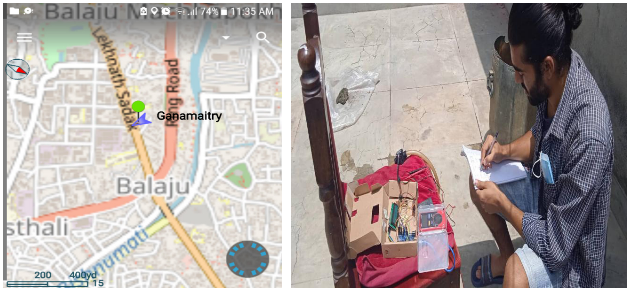
Figure 8. Data collection using device in Balaju area
