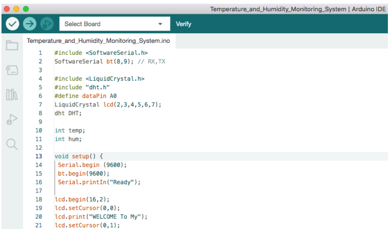
Figure 5. Arduino software
