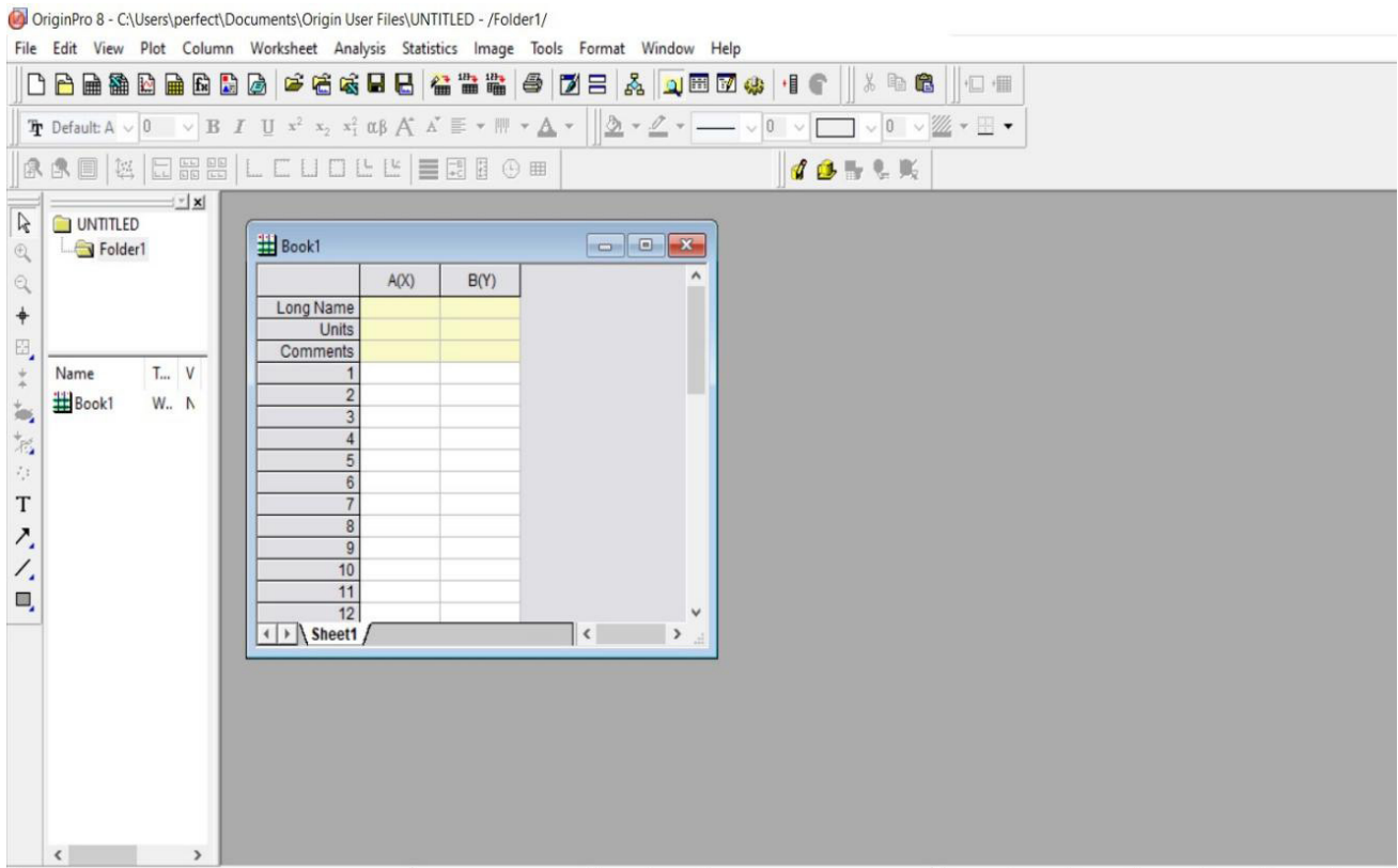
Figure 6. Origin Software
