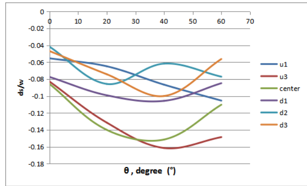
Figure 14. Variation of Scour along different Angular Displacement and different sections for front pier along longitudinal centerline
