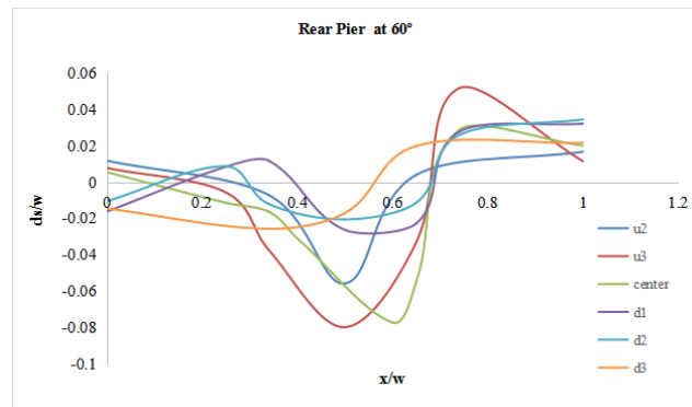
Figure 11. Variation of Scour along different sections of rear pier when front pier placed at 60^\circ
