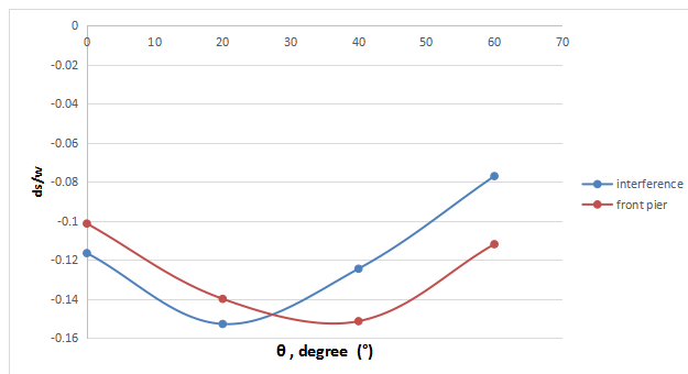
Figure 17. Comparison between scour of rear and front pier at different angular displacements at center section at 40^\circ .
