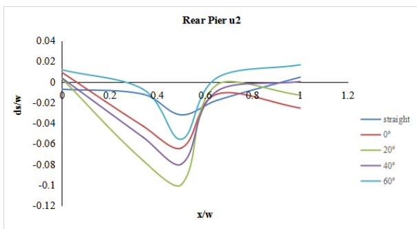
Figure 13. Variation of Scour of rear pier for different Angular Displacement of front pier at u2 section
