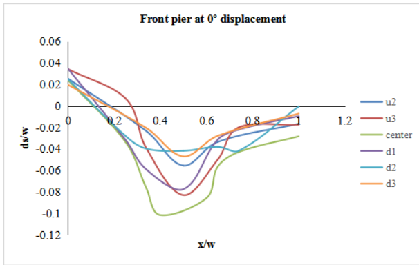
Figure 8. Variation of Scour along different sections of front pier when placed at 0^\circ
