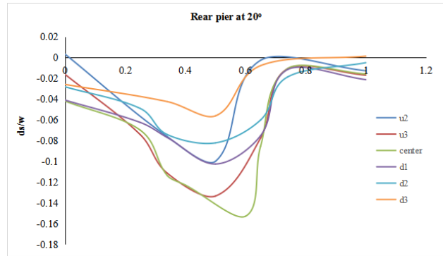
Figure 10. Variation of Scour along different sections of rear pier when front pier placed at 20^\circ
