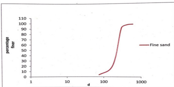
Figure 3. Particle size Distribution Curve
