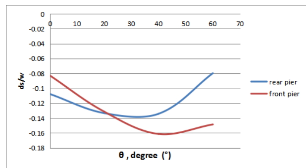
Figure 15. Comparison between maximum scour between rear pier and front pier at different angular displacements Figure 16 shows the variation of scour of front pier at
