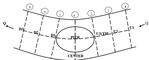
Figure 7. Position of Pier in Bend - 2 and various Sections under consideration
