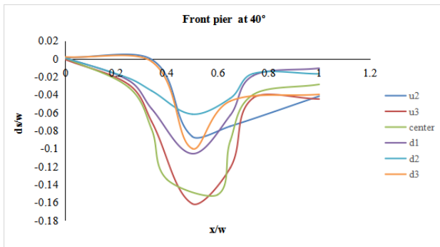
Figure 9. Variation of Scour along different sections of front pier when placed at 40^\circ
