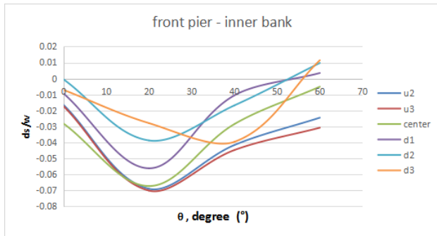
Figure 16. Variation of Scour along different Angular Displacement and different sections for front pier at inner bank
