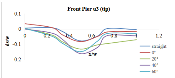
Figure 12. Variation of Scour of front pier for different Angular Displacement at u3 (tip) section
