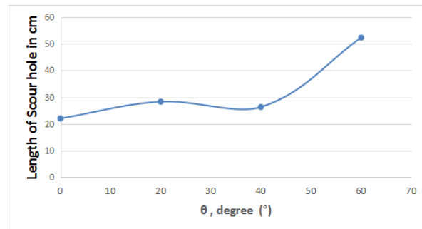
Figure 18. Variation of longitudinal length of scour hole of rear pier due to change in angular displacement of front pier
