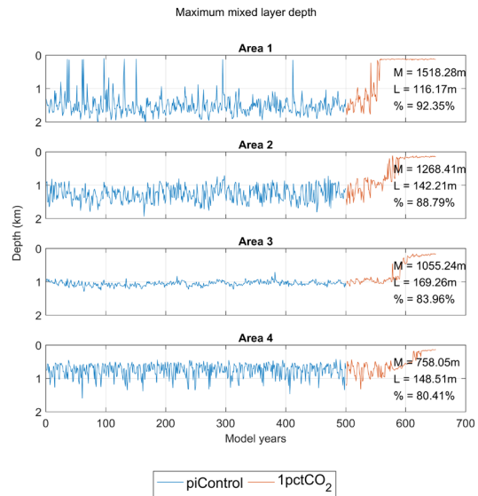
Figure 6. Time series of maximum mixed layer depth in March for each area (red polygons in Figure 1) in the piControl and 1pctCO 2 experiments. M represents the average piControl value, L is the average L-1pctCO 2 value, and % indicates the percentage of shallowing (decrease in mixed layer depth) in L-1pctCO 2 compared to the time average of 500 years of piControl. Shallowing refers to a reduction in the maximum depth of the mixed layer, which measures the depth of the layer in which temperature and salinity are relatively uniform.
