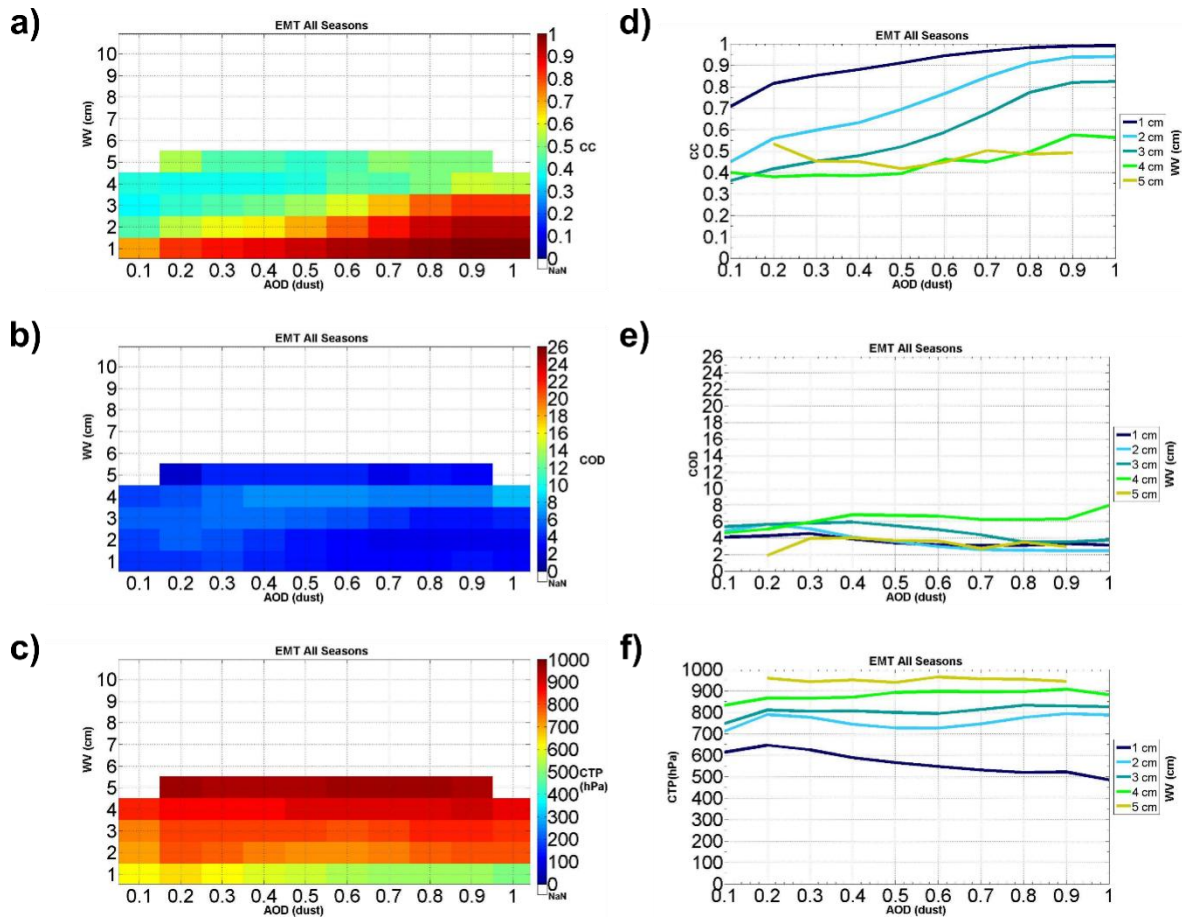
Figure 9. Mean dust Aerosol Optical Depth at 550 nm (AOD dust )-Water Vapor (WV)-Cloud Cover (CC) relationships (a,d), mean dust Aerosol Optical Depth at 550 nm (AOD dust )-Water Vapor (WV)-Cloud Optical Depth (COD) relationships (b,e) and mean dust Aerosol Optical Depth at 550 nm (AOD dust )-Water Vapor (WV)-Cloud Top Pressure (CTP) relationships (c,f), over the Eastern Mediterranean for all seasons, from Aqua, for the period 2002–2012. Figures on the left present results in bins, while figures on the right present results as line graphs. The data were sorted into 0.1 (AOD dust ) and 1 cm WV bins to minimize the effect of spatial heterogeneity of local meteorology. The color bars represent the average CC, COD and CTP values in each (AOD dust ) and WV bin. NaN at the color bars denote less than 30 values in this bin.
