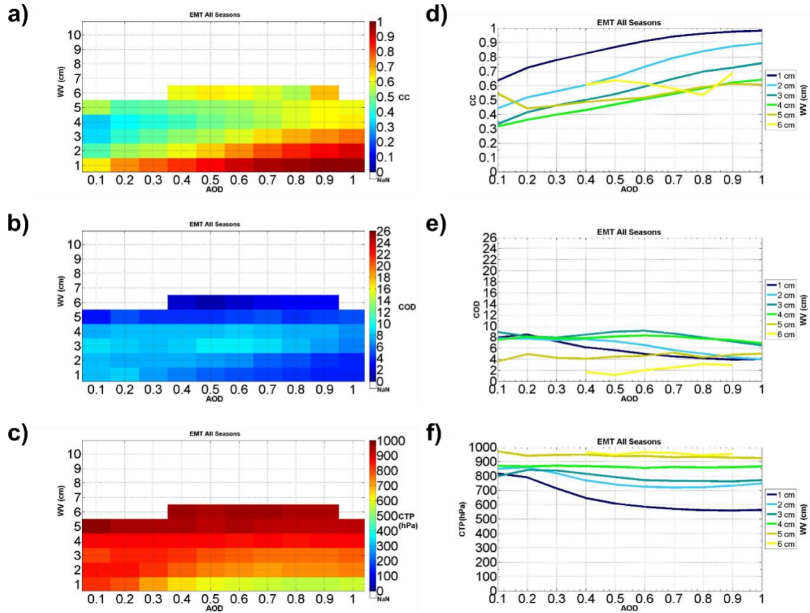
Figure 3. Mean total Aerosol Optical Depth at 550 nm (AOD)-Water Vapor (WV)-Cloud Cover (CC) relationships ( a,d ), mean total Aerosol Optical Depth at 550 nm (AOD)-Water Vapor (WV)-Cloud Optical Depth (COD) relationships ( b,e ) and mean total Aerosol Optical Depth at 550 nm (AOD)-Water Vapor (WV)-Cloud Top Pressure (CTP) relationships ( c,f ), over the Eastern Mediterranean for all seasons, from Aqua, for the period 2002–2012. Figures on the left present results in bins, while figures on the right present results as line graphs. The data were sorted into 0.1 AOD and 1 cm WV bins to minimize the effect of spatial heterogeneity of local meteorology. The color bars represent the average CC, COD and CTP values in each AOD and WV bin. NaN at the color bars denote less than 30 values in this bin.
