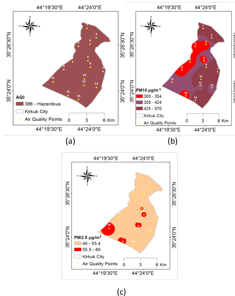
Figure 3. Air quality spatial distributions in Kirkuk city from April 2022 to January 2023: (a) AQI, (b) PM10, (c) PM2.5.
