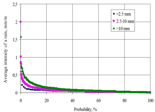
Figure 5. Availability of average precipitation intensity at the weather station Kamenka-Bugskaya is differentiated by the amount of precipitation per rain.
