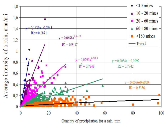
Figure 9. Dependence of the intensity of precipitation on their amount, differentiated in more detail by the duration of rain, meteorological station Kamenka-Bugskaya.
