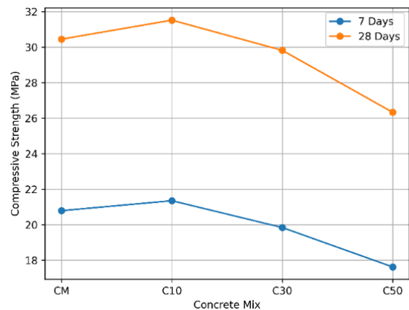
Figure 4. Comparison between compressive strength development of recycled aggregate concrete on 7 and 28 days.
