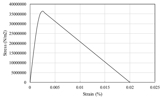
Figure 2. Uniaxial compression model.
