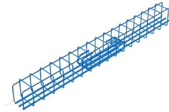
(c) Beam with hooked-end bar lap splices.
