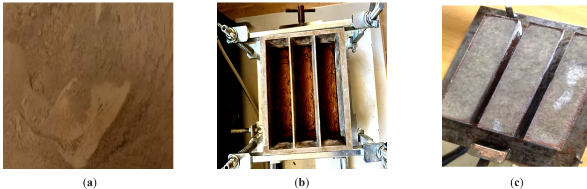
Figure 3. Preparation of clay-biopolymer composite bricks: (a) Powdered clay-biopolymer composite; (b) Mold (dimensions: 160 mm \times 40 mm \times 40 mm); and (c) Molded clay-biopolymer composites.
