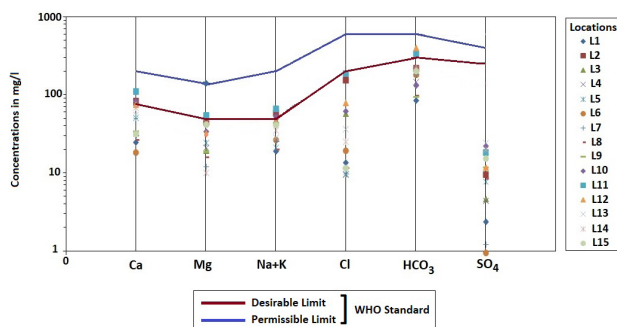
Figure 7. Schoeller Diagram
