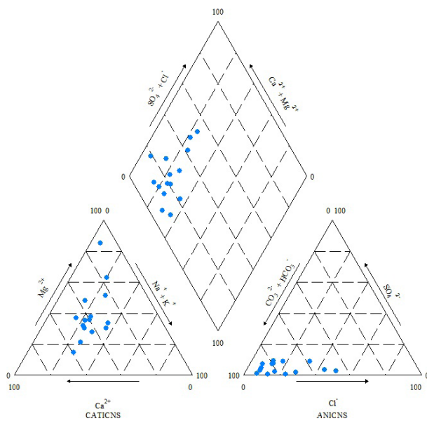
Figure 6. Piper Diagram
