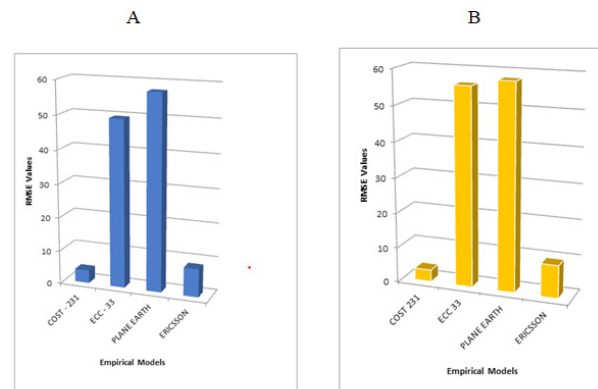
Figure 7. A bar chart representing the root mean square error (RMSE) values for MTN 3G.
