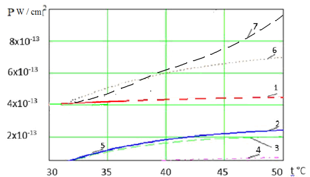
Figure 9. The graph of the integrated power changes
