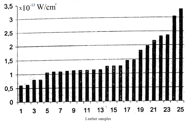
Figure 13. Distribution of own radiation of skin samples
