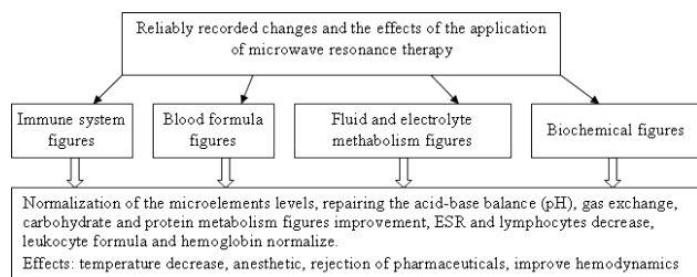
Figure 5. Effects of Quantum Medicine
