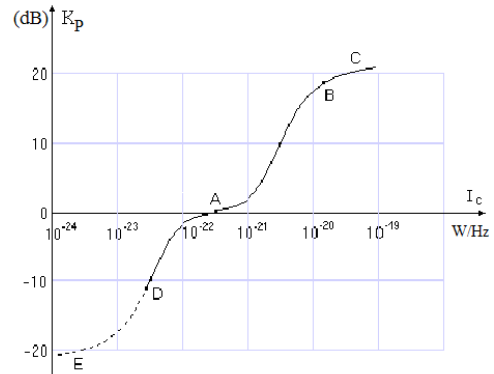
Figure 11. Distribution of the human palm absorbance ability in contact with the positive and negative EMR flows
