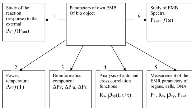
Figure 7. Classification of measuring tasks in the study of the bioobject own EMR
