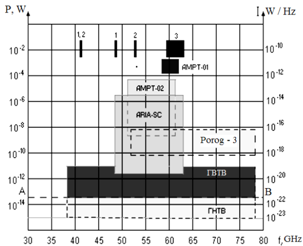
Figure 1. Distribution of power and frequency range of devices
