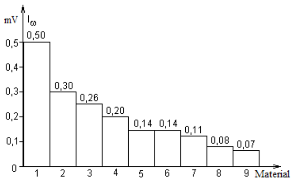
Figure 12. Distribution emissivity of textile materials for clothes
