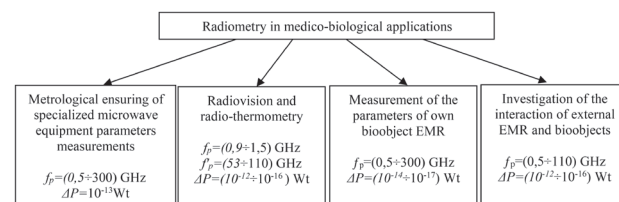
Figure 6. Classification of radiometric problems in the medical and biological applications
