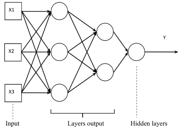
Figure 2. Multi-layer perceptron
